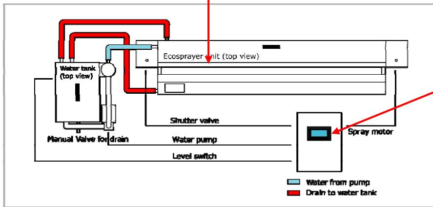
connection diagram of Ecosprayer unit
